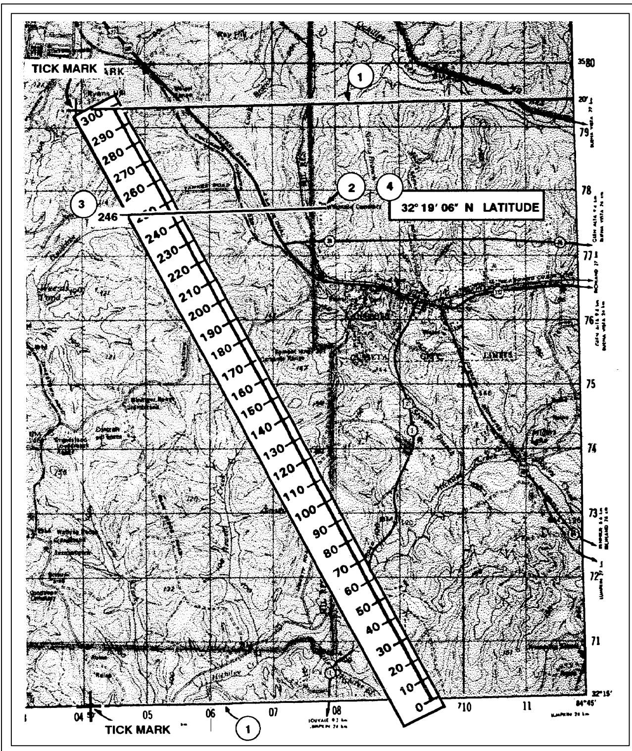
Figure 4-4. Determining latitude.
