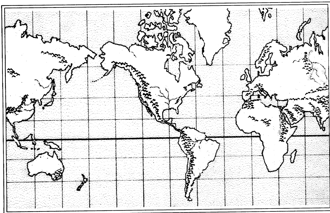
Figure 13-2. Mountain systems.
